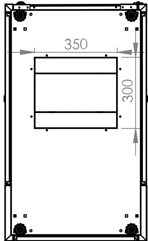
Bottom view
