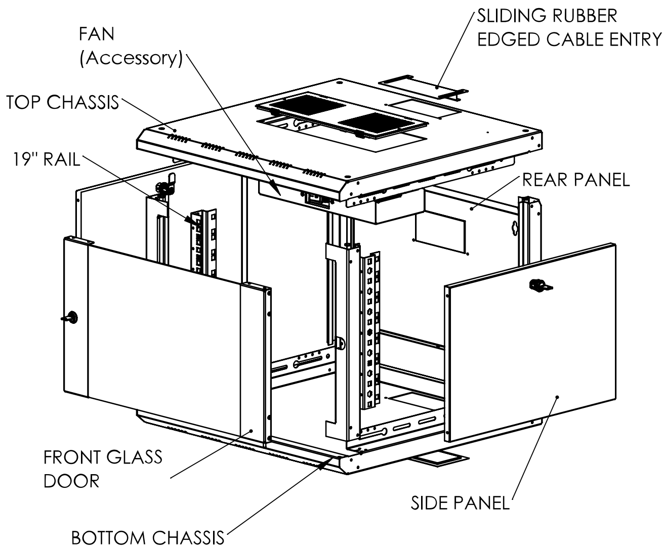
Exploded view
